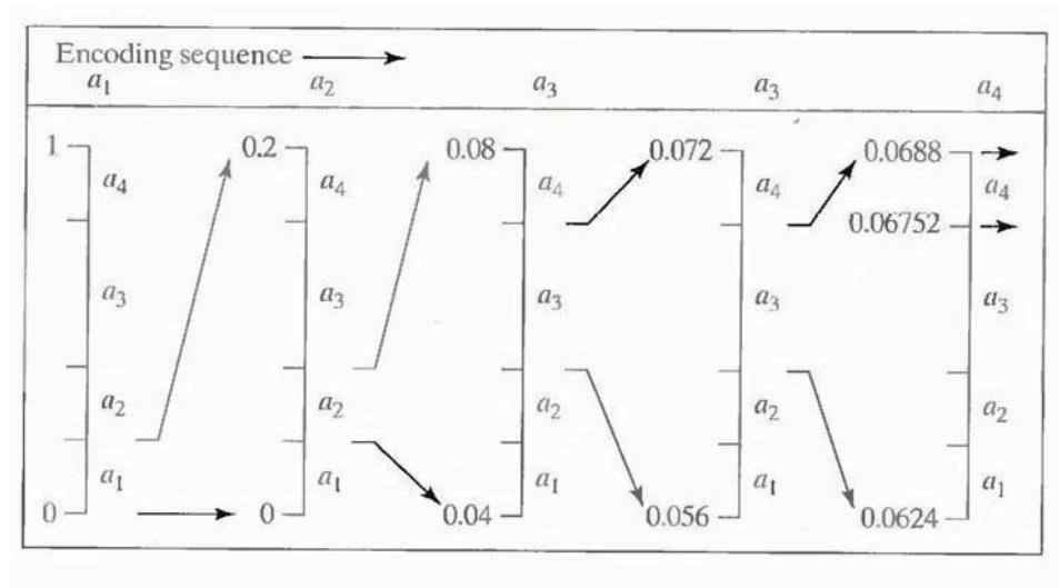
Fig.5.1 Arithmetic coding procedure
